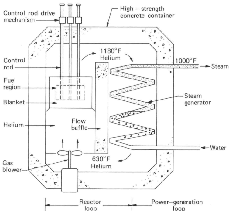
Figure 5 GCFR nuclear steam supply.
