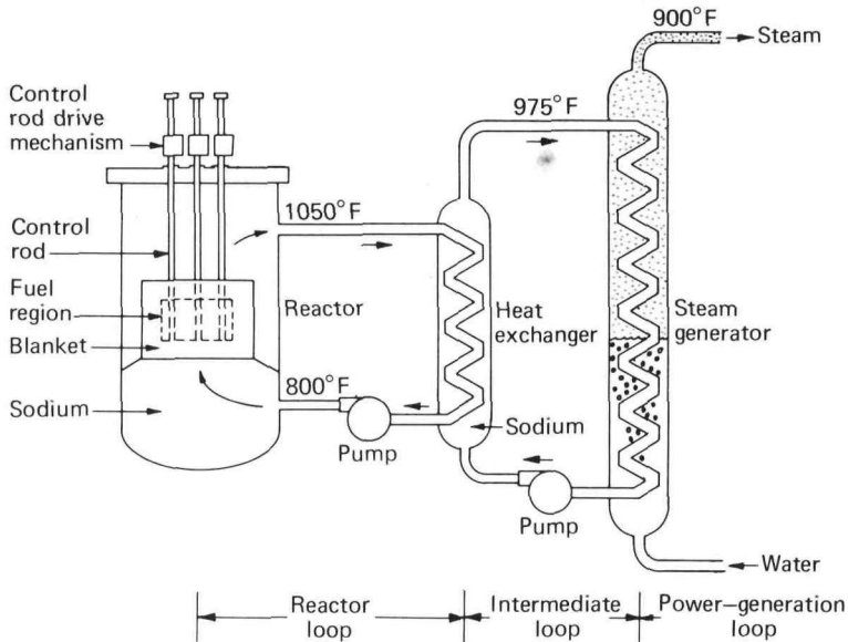
Figure 3 LMFBR nuclear steam supply.
