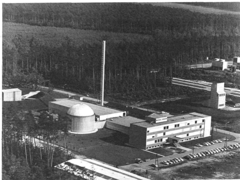
Figure 18 The zero-power reactor SNEAK.
