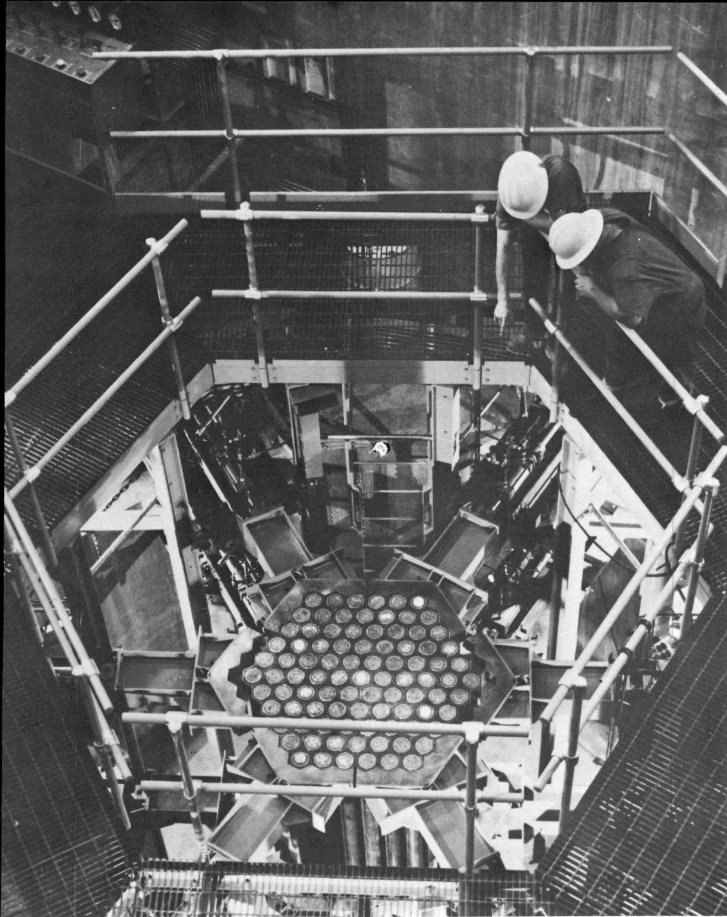
Figure 2 The Fast Flux Test Facility (FFTF), now under construction at the AEC's Hanford Works in the State of Washington, will be a key part of LMFBR development. In the photograph engineers discuss operation of the simulated core mockup of the FFTF. (See page 30.)
