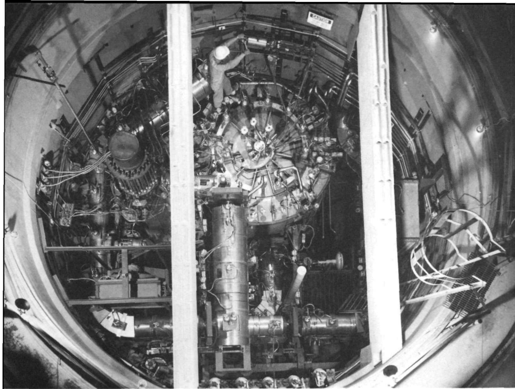
Figure 7 A technician stands atop the thermal shield of the Molten Salt Reactor during the reactor's installation.
