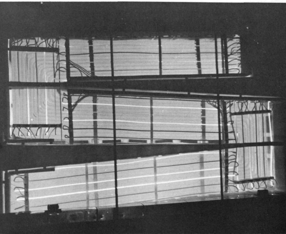
Figure 8 Primary heat exchanger of the Molten Salt Reactor has a heat-transfer area of nearly 259 square feet. Heat is removed from the coolant-salt mixture in the air-blast radiator and is dissipated through a metal stack to the atmosphere. The coolant flows through tubes \frac{3}{4} inch in diameter and 30 feet long. The tubes are arranged in 10 banks with 12 tubes in each bank. The photograph was taken with the light emitted from the molten salt mixture.
