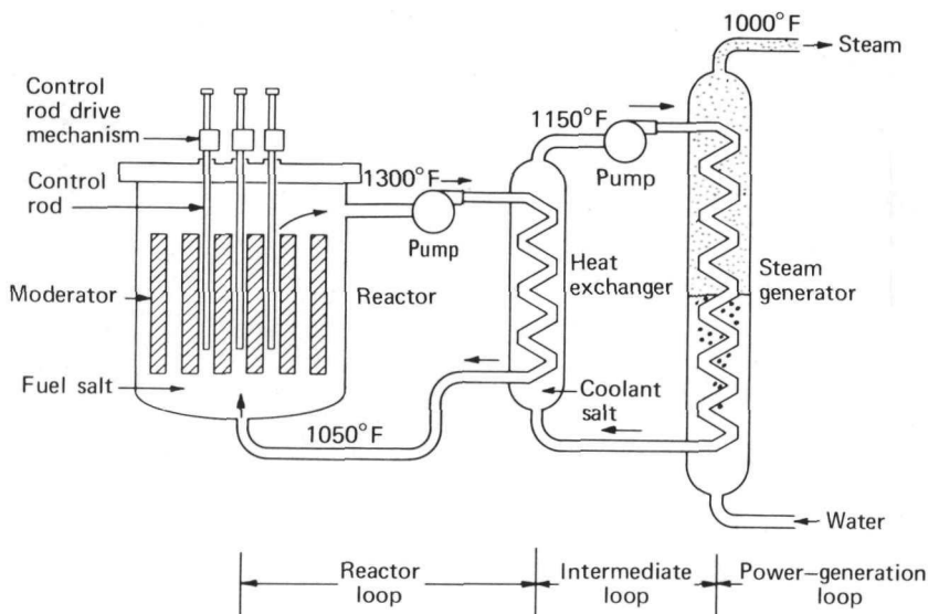
Figure 6 MSBR nuclear steam supply.
