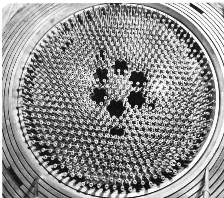
Figure 16 The core of Rapsodie reveals the numerous core assemblies of this small reactor.
