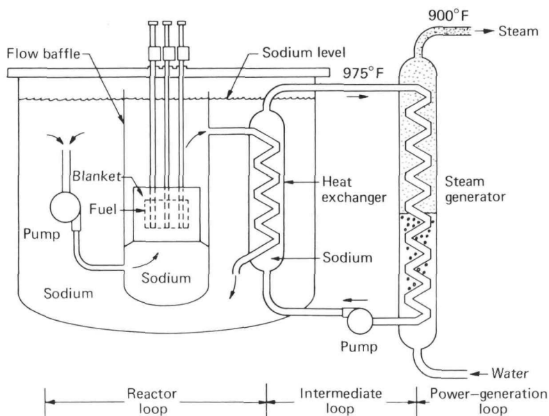
Figure 4 Pot-type LMFBR nuclear steam supply.
