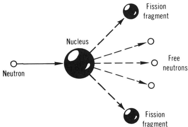
Figure 1 A fission reaction.
