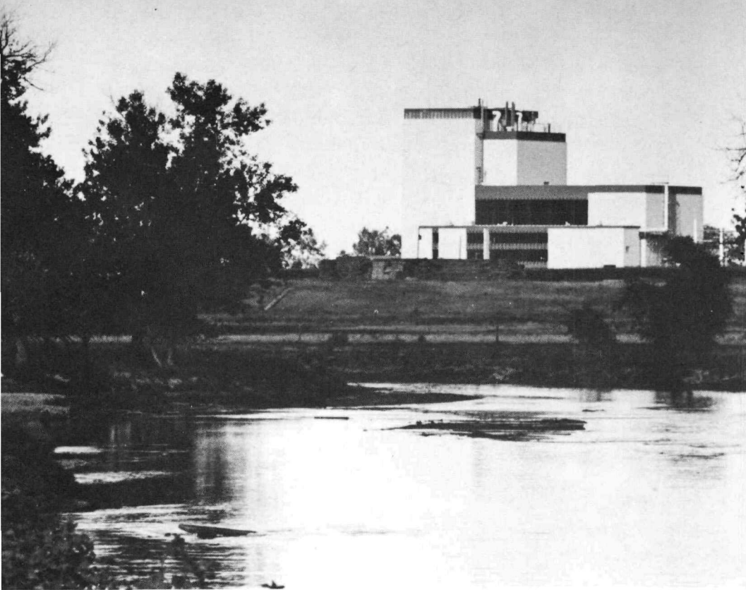
Figure 21 The Fort St. Vrain Nuclear Generating Station under construction at Platteville, Colorado, will be a high-temperature, gas-cooled thermal reactor (HTGR). It operates on a thorium-uranium fuel cycle and uses helium as a coolant. Experience with this reactor will contribute a great deal to breeder reactor development because helium has special advantages as a coolant for fast breeder reactors.
