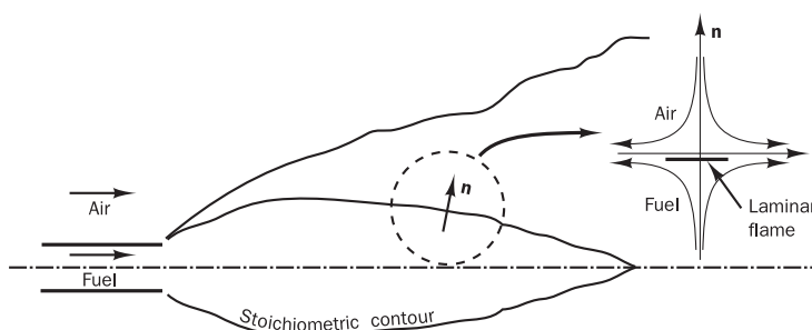
Figure 12.11 Schematic representation of the laminar flamelet concept
