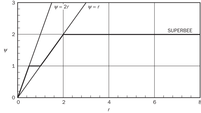
Figure D.4 SUPERBEE limiter
